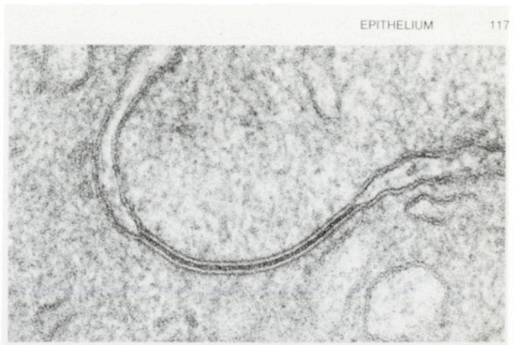
Fig. 4-12. High magnification electron micrograph showing a communicating (gap) junction between two adjacent liver cells of a rat. The cell membranes of neighboring hepatocytes comes into very close proximity in a region shown in the center of the micrograph. Close inspection discloses a 20- to 40-Å gap between the membranes in this region. \times 220,000 . (Courtesy of Dr. Norton B. Gilula.)
